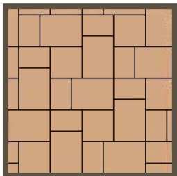
Pattern 1 53% 9 x 12 - 20% 9 x 9 - 27% 6 x 9
